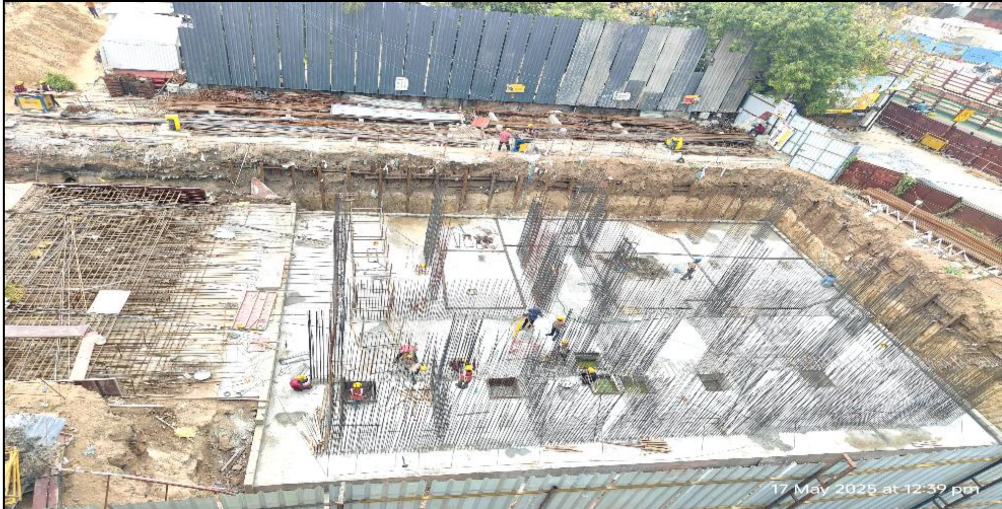
STP – Raft concrete work completed
