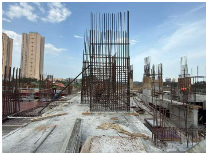
Column Reinforcement
