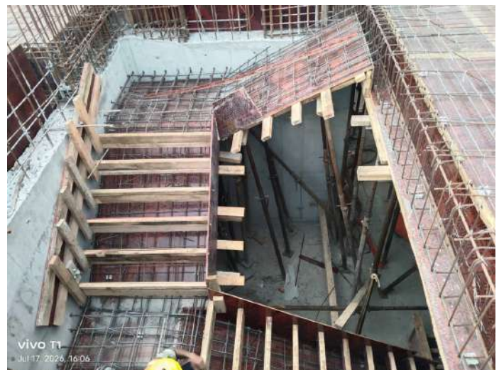
Staircase Reinforcement
