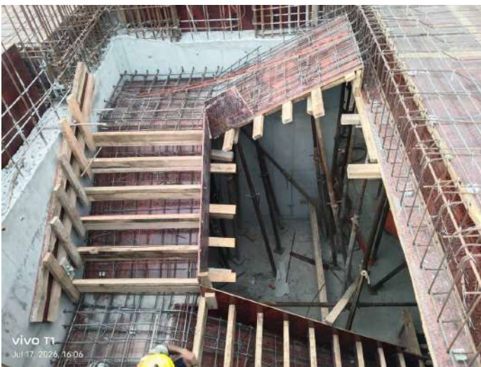
Staircase Shuttering
