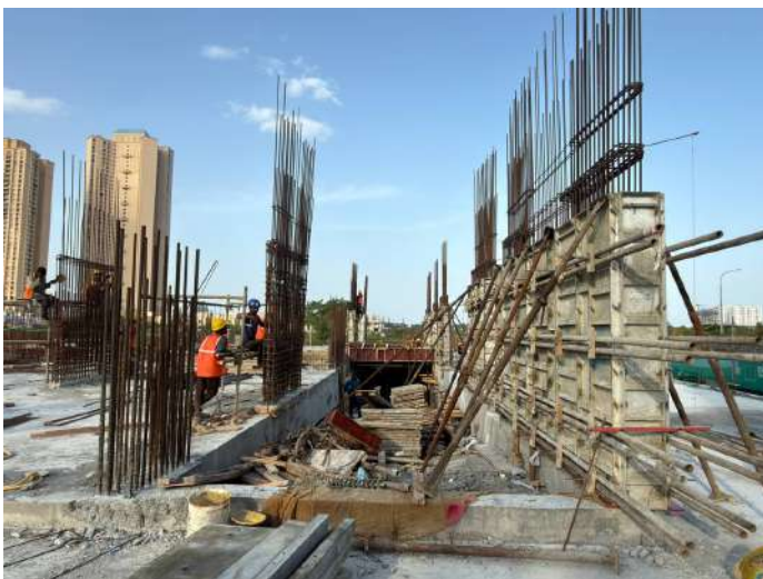
Column Reinforcement
