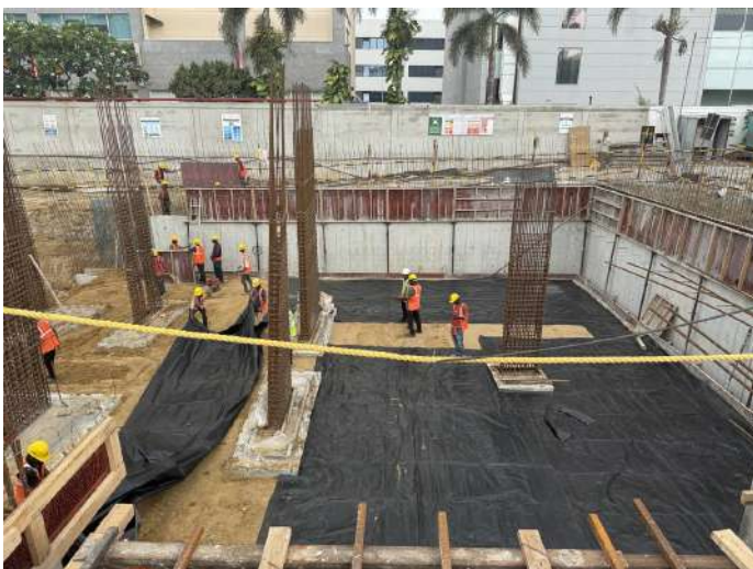
Grade Slab PCC
