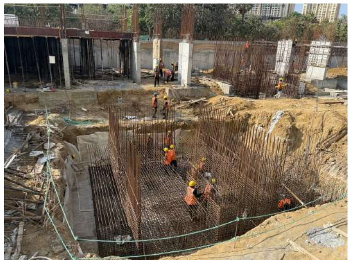
Raft & Pilecap Steel Reinforcement
