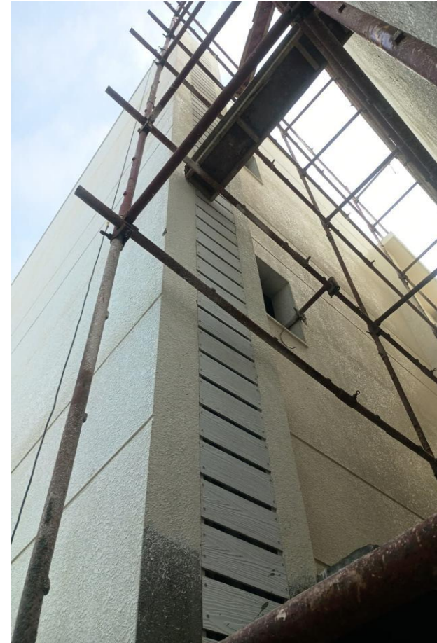
Villa 17 Plumbing Shaft Cera Board Fixing Completed
